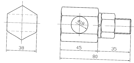
01 SIDE BRACING ASS'Y
